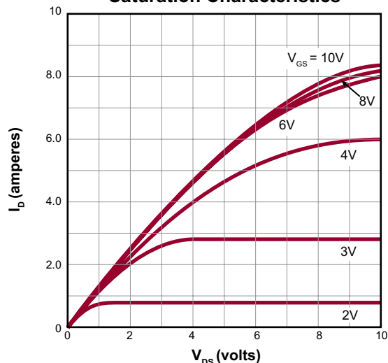
Saturation Characteristics
