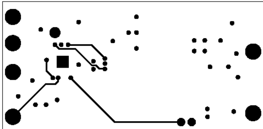
FIGURE 16. ISL6406EVAL2 - LAYER 4
