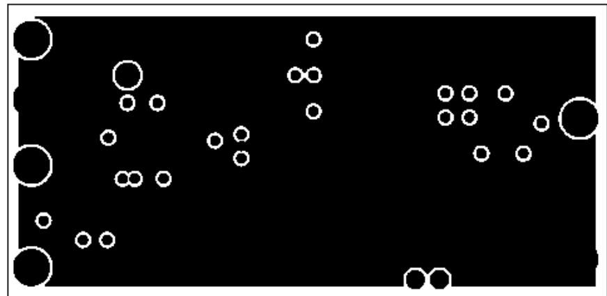
FIGURE 14. ISL6406EVAL2 - LAYER 2
