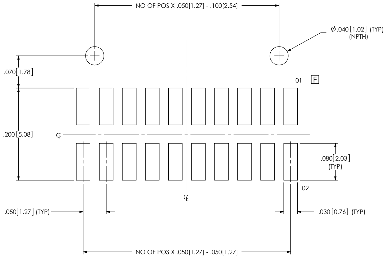
FIG 1 FTSH-110-XX-XXX-DH-A SHOWN
