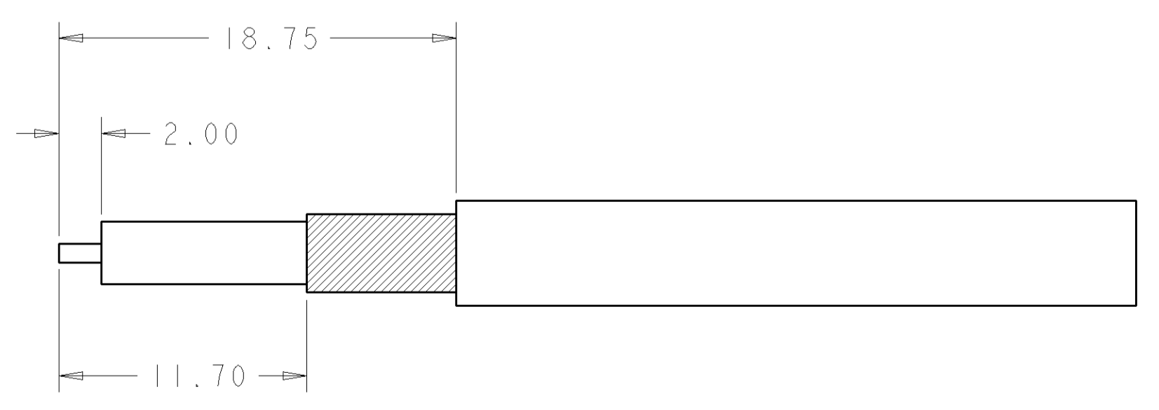
RECOMMENDED STRIP LENGTHS SCALE 4:1
