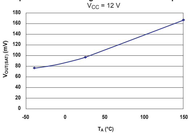
Output Saturation Voltage versus Ambient Temperature
