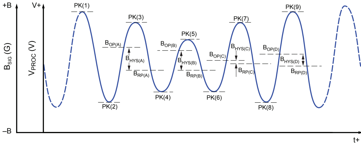
Figure 5. The Continuous Update algorithm operation. Not detailed in the figure are the boundaries for peak capture DAC movement which intentionally limit the amount of inward signal variation the IC is able to react to over a single transition. The algorithm is used to establish and subsequently update the device switchpoints ( B_{OP} and B_{RP} ). The hysteresis, B_{HYS(\#x)} , at each target feature configuration results from this recalibration, ensuring that it remains properly proportioned and centered within the peak-to-peak range of the internal analog signal, V_{PROC} .
