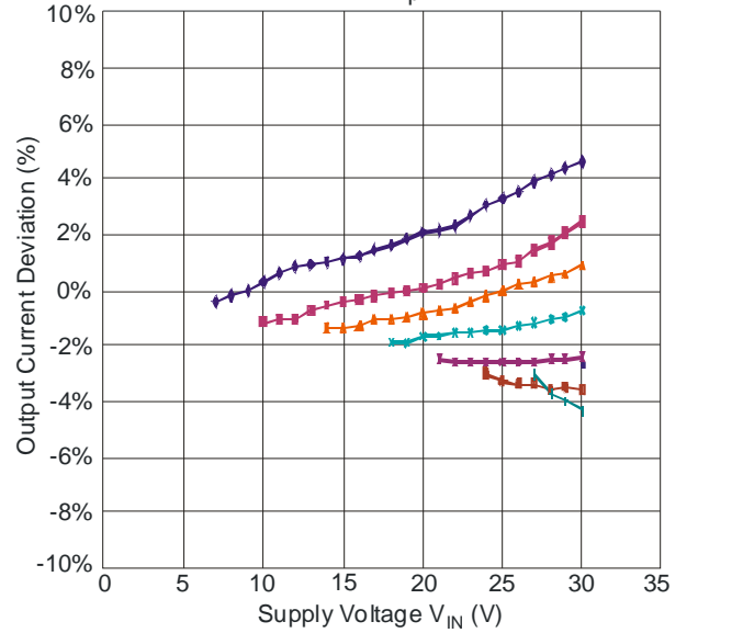
ZXLD1360 Output Current L = 47µH
