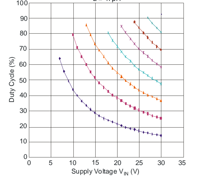
ZXLD1360 Duty Cycle L = 47µH
