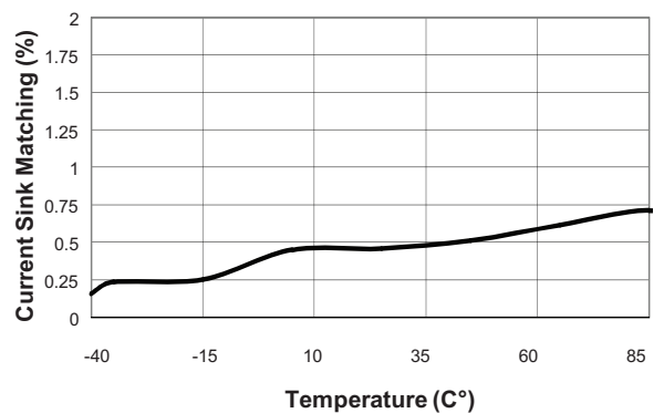
Current Sink Matching vs Temperature ( V_{IN} = 12V ; 30mA/ch)
