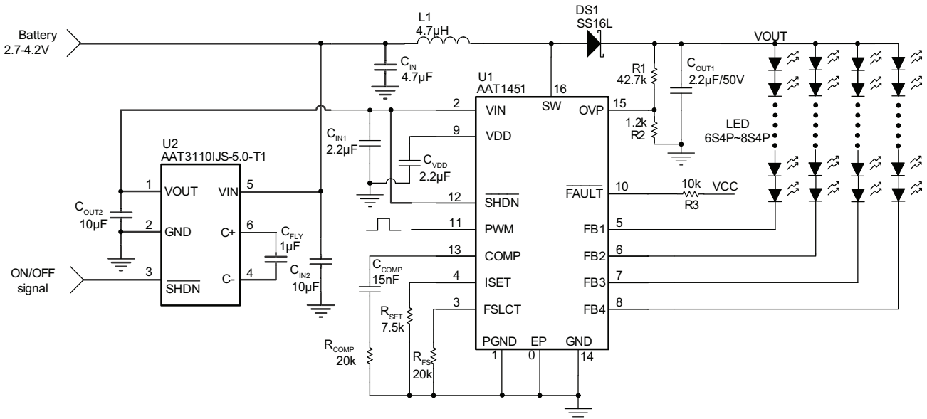
Figure 7: Schematic of AAT1451 plus AAT3110
