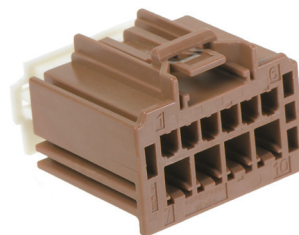
Series 34969, 14-circuit hybrid female receptacle
