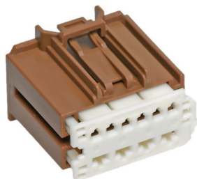
Series 34969, 14-circuit hybrid female receptacle
