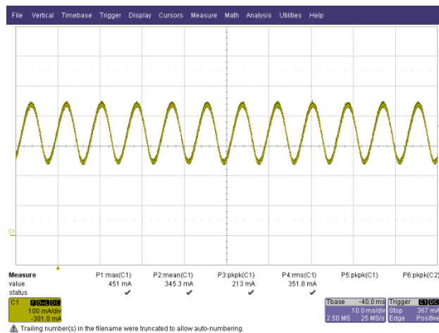
Figure 37 – 100 VAC, 60 Hz Full Load. I OUT , 100 mA / div., 10 ms / div.
