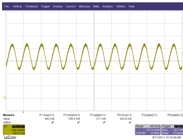
Figure 36 – 90 VAC, 60 Hz Full Load. I OUT , 100 mA / div., 10 ms / div.
