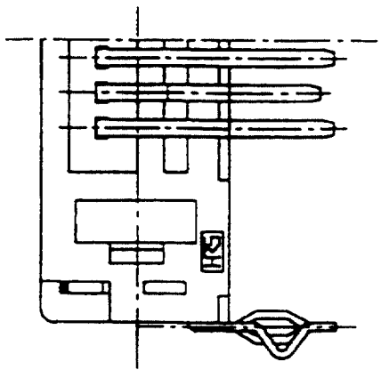
RECOMMENDED PC BOARD PATTERN (2/1) (MOUNTING SIDE)
