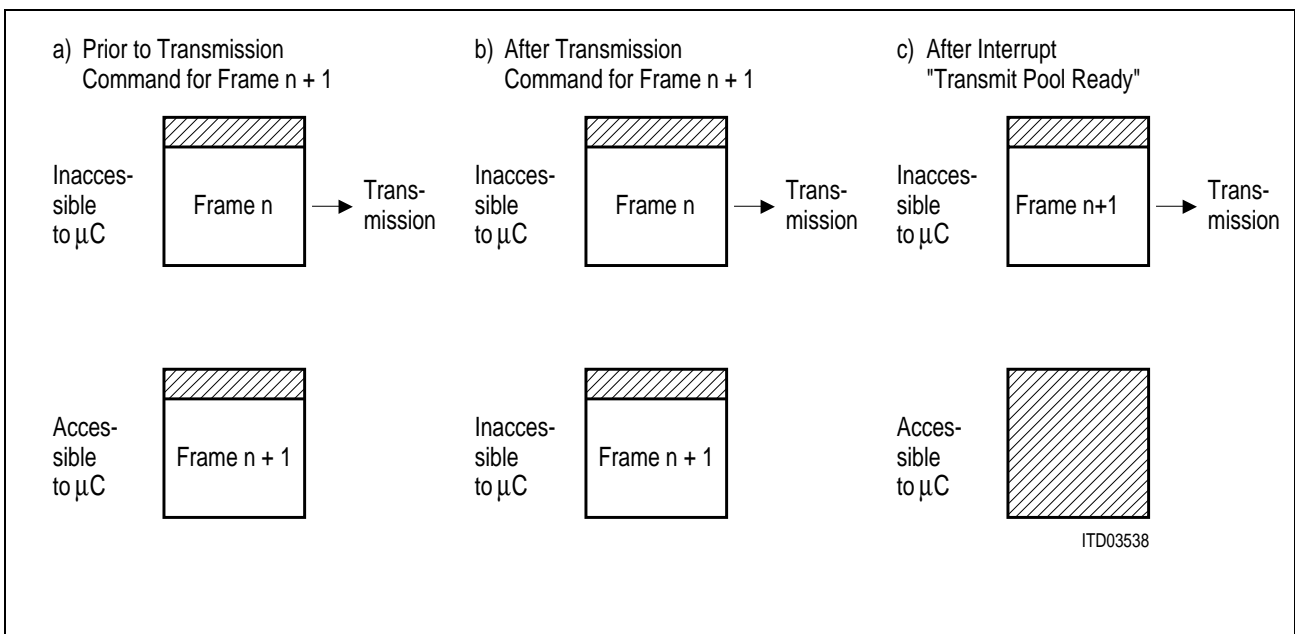
Figure 11 Transmit FIFO
