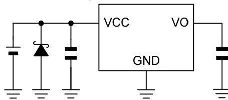
Figure 26. Application Example 2
