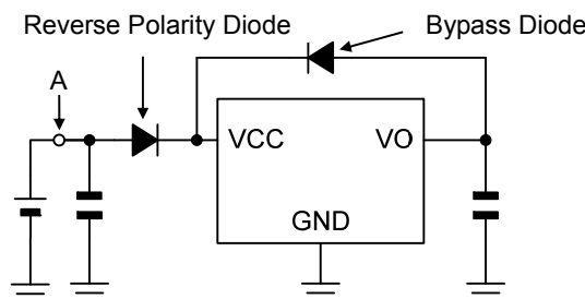
Figure 28. Application Example 4
