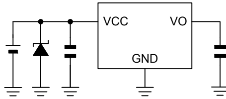
Figure 25. Application Example 1
