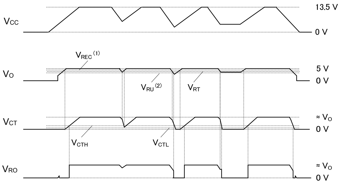
Figure 21. Timing Chart
