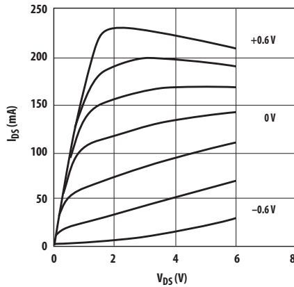
Figure 1. Typical/Pulsed I-V Curves [6] . ( V_{GS} = -0.2V per step)
