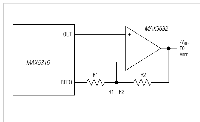
Figure 12. Bipolar Output
