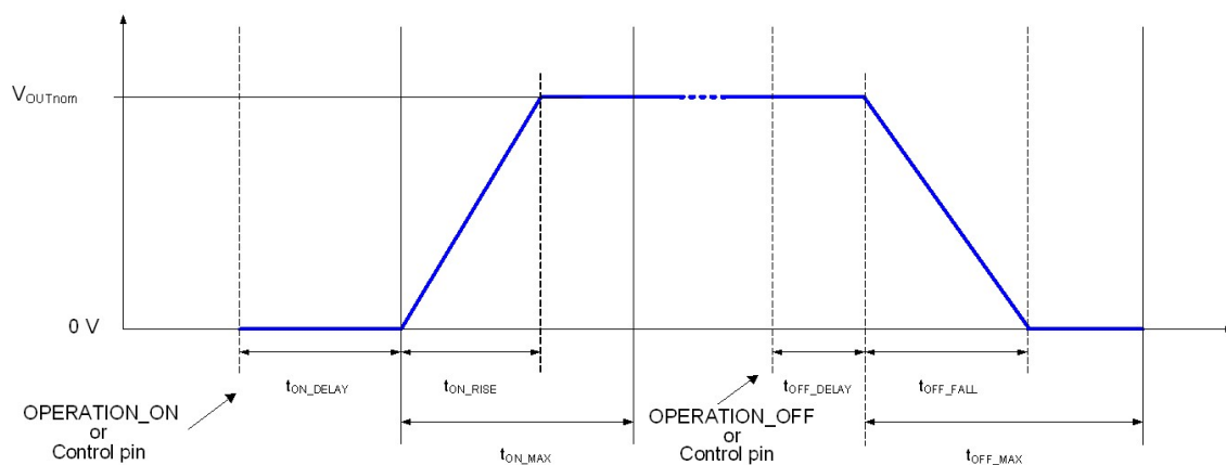
Figure 5: Power Sequencing
