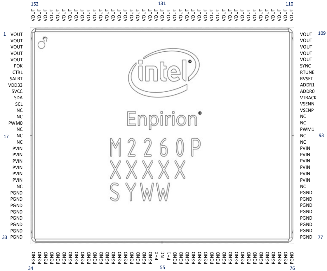
Figure 1: Pin Out Diagram (Top side)
