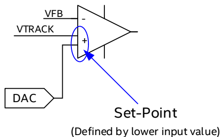
Figure 8: VTRACK Circuitry
