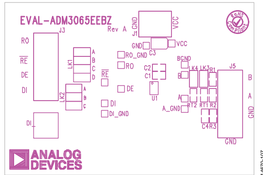
Figure 7. EVAL-ADM3065EEBZ/EVAL-ADM3065EEB1Z Silkscreen
