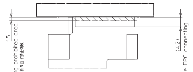
DETAIL B (2:1)
