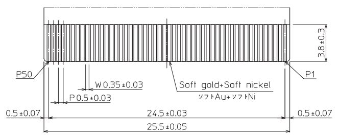
DETAIL C (5:1)
