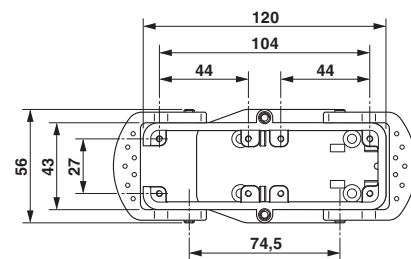
Dimensional drawing, a = 120 mm
