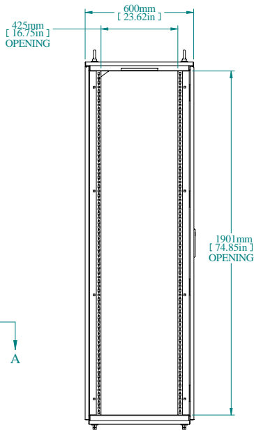
L.S. VIEW
