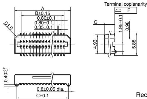
General tolerance: ±0.3
