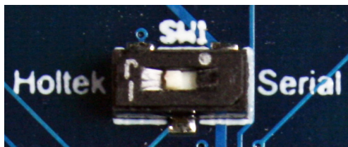
Figure 6: The Evaluation Board Protocol Selection Switch
