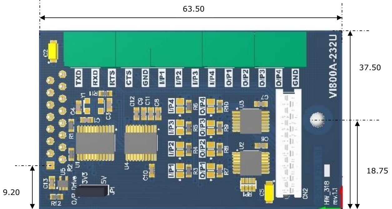
Figure 3-2 - VI800A-232U module PCB Top view
