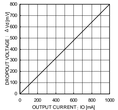
Fig.6 Dropout Voltage ( V_{cc}=V_o \times 0.95\text{V} ) ( I_o=0\text{mA} \rightarrow 1000\text{mA} )
