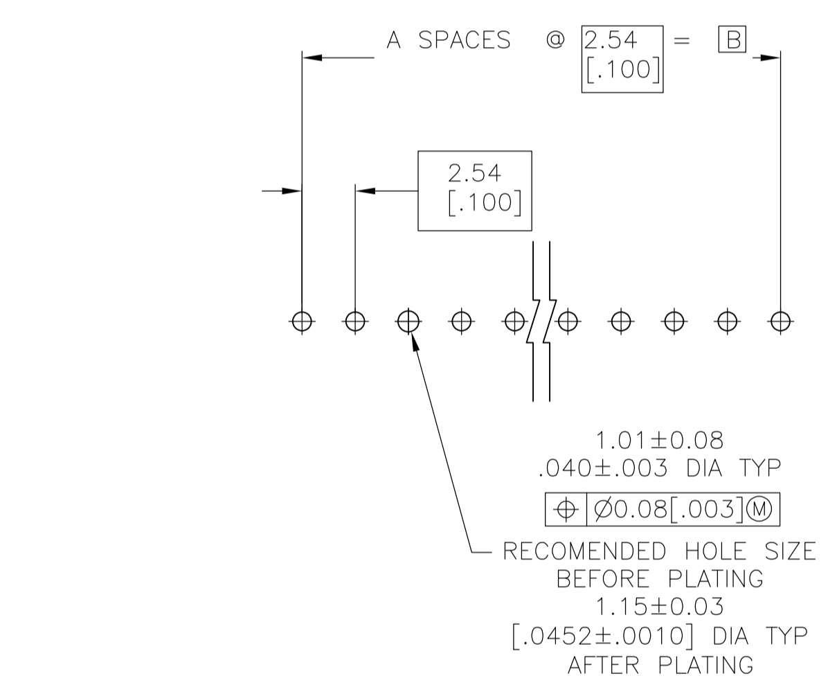
RECOMMENDED PC BOARD MOUNTING DIMENSIONS
