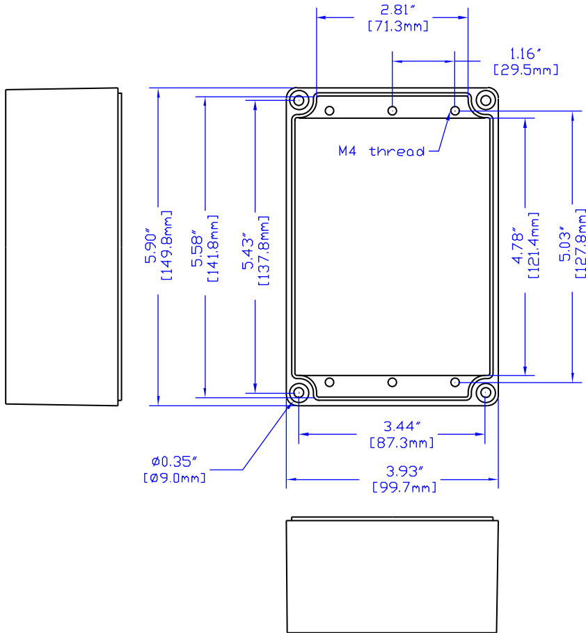
VIEW OF BOX (LID REMOVED)
