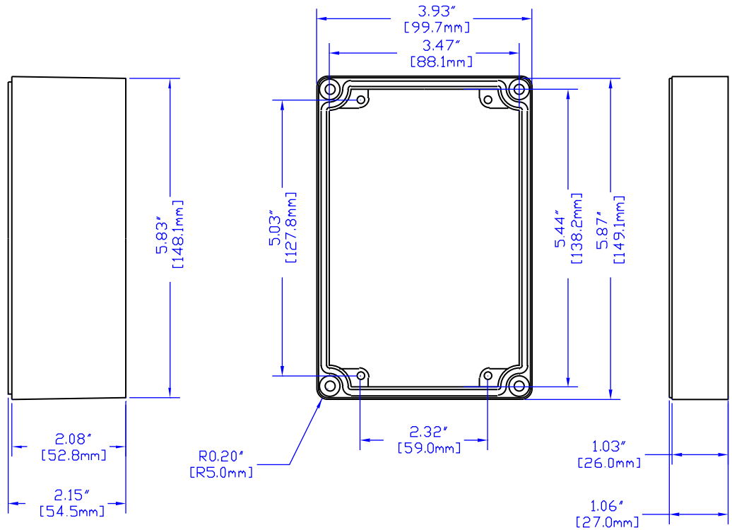
VIEW OF LID (INSIDE)
