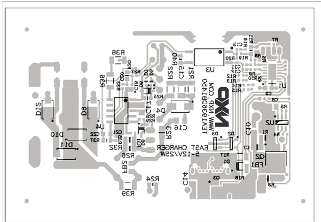
Figure 29. Bottom copper and top silk screen (mirrored)
