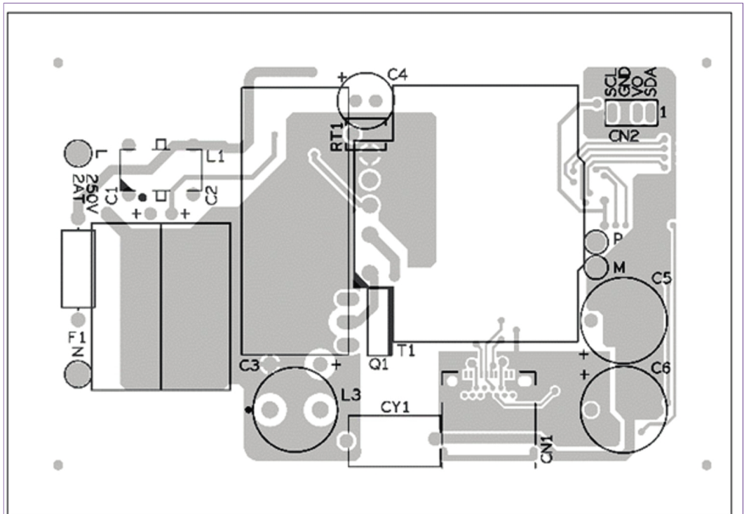
Figure 28. Top copper and top silk screen
