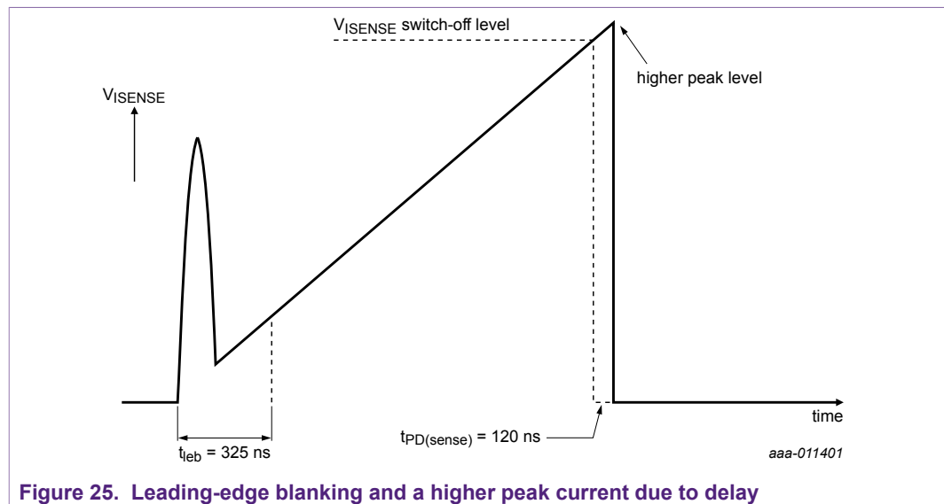
Figure 25. Leading-edge blanking and a higher peak current due to delay
