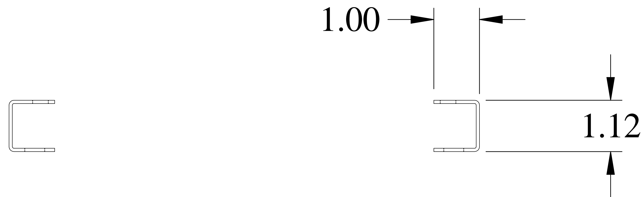
BOTTOM VIEW
