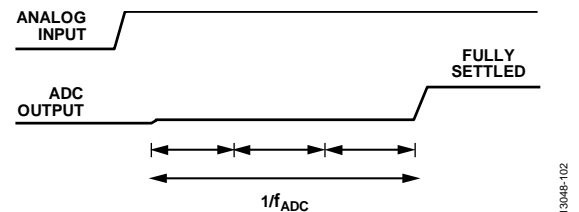
Figure 95. Sinc 3 Zero Latency Operation
