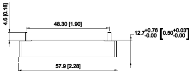
Figure 21 the pin function and mechanical drawing
