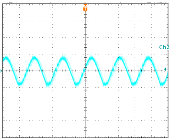
Figure 10: Output voltage ripple at nominal input voltage and max load current (10 mV/div, 2 \mu s /div) Bandwidth: 20 MHz.
