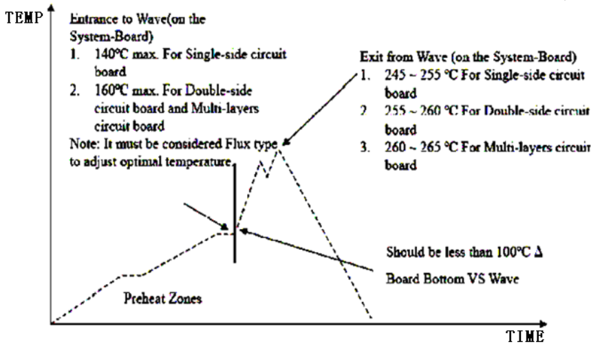
Figure 19 recommended temperature profile for lead-free wave soldering
