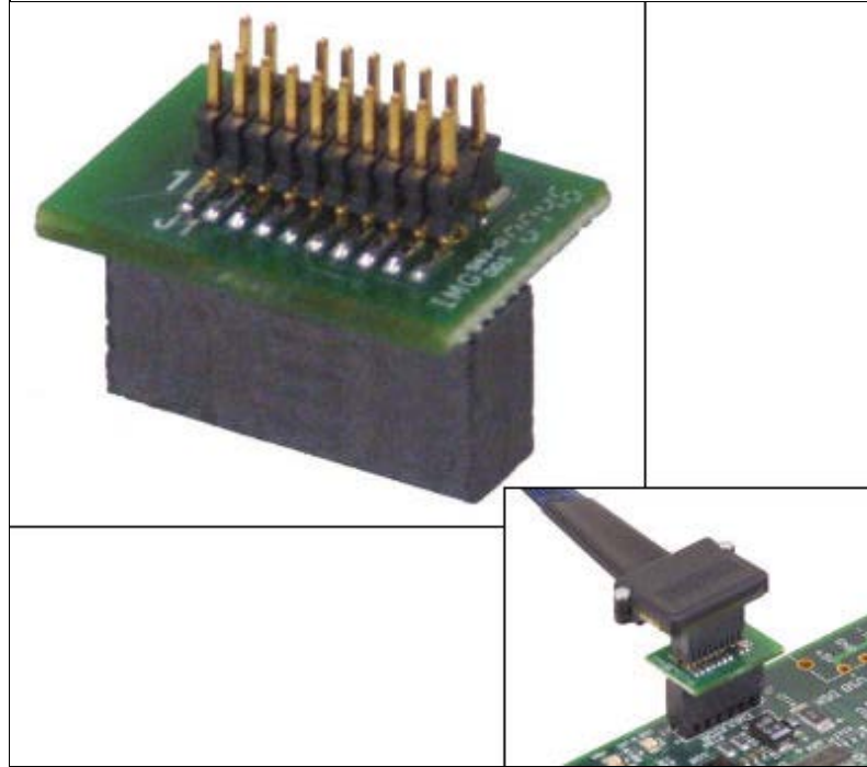
20-pin CTI to 14-pin JTAG Adapter
