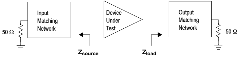
Figure 12. Series Equivalent Source and Load Impedance – 2700–3100 MHz
