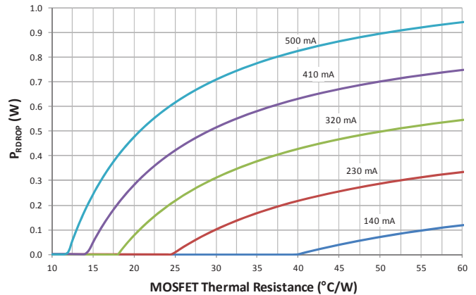
Figure 9. R_{DROP} Dissipation versus MOSFET thermal resistance at various V33 regulator maximum current settings, I_{V33ILIM}
