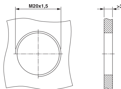
Installation dimensions
