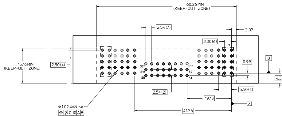
RECOMMENDED PC BOARD LAYOUT & KEEP-OUT ZONE
